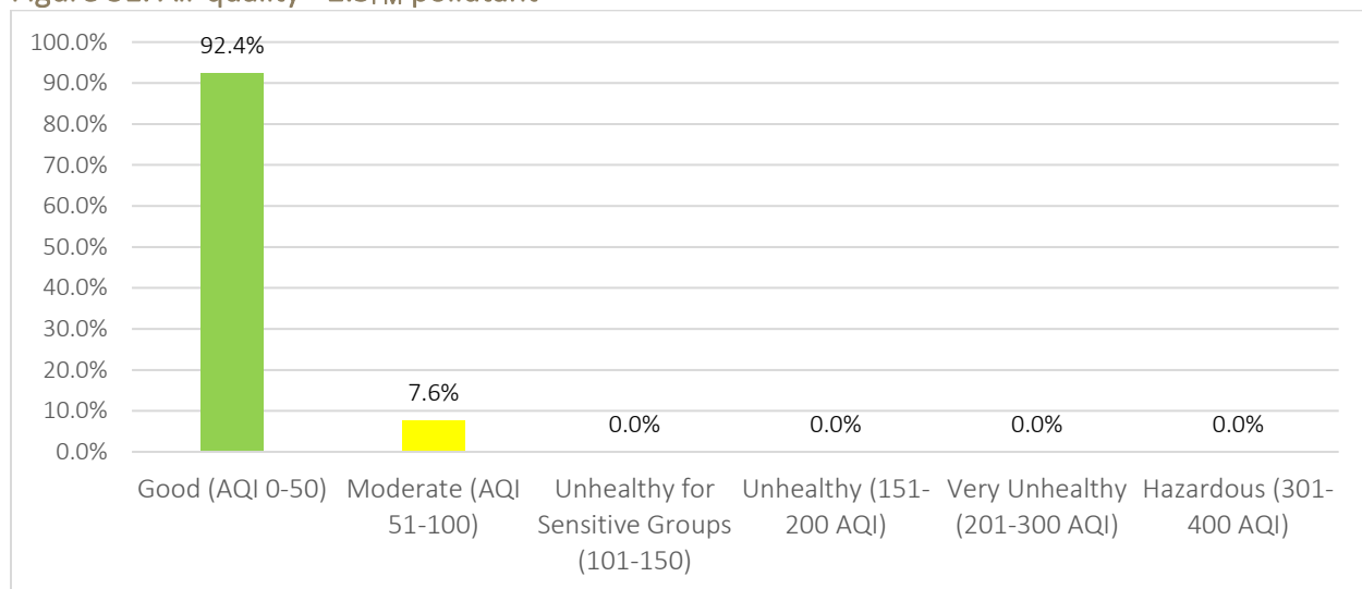
Figure 31. Air quality - 2.5 PM pollutant
