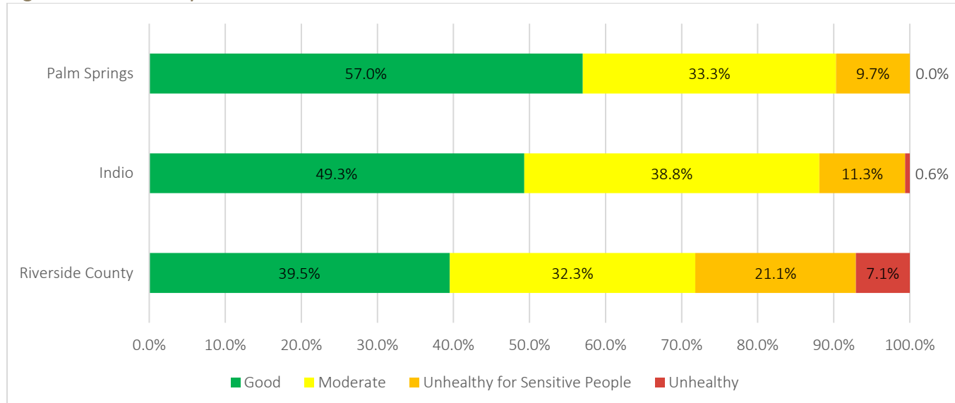
Figure 33. Air Quality Based on Ozone Pollution
